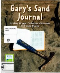
Investigating Sand
