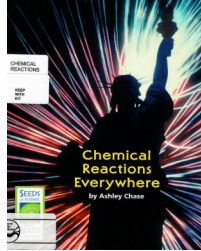
Chemical Reactions
